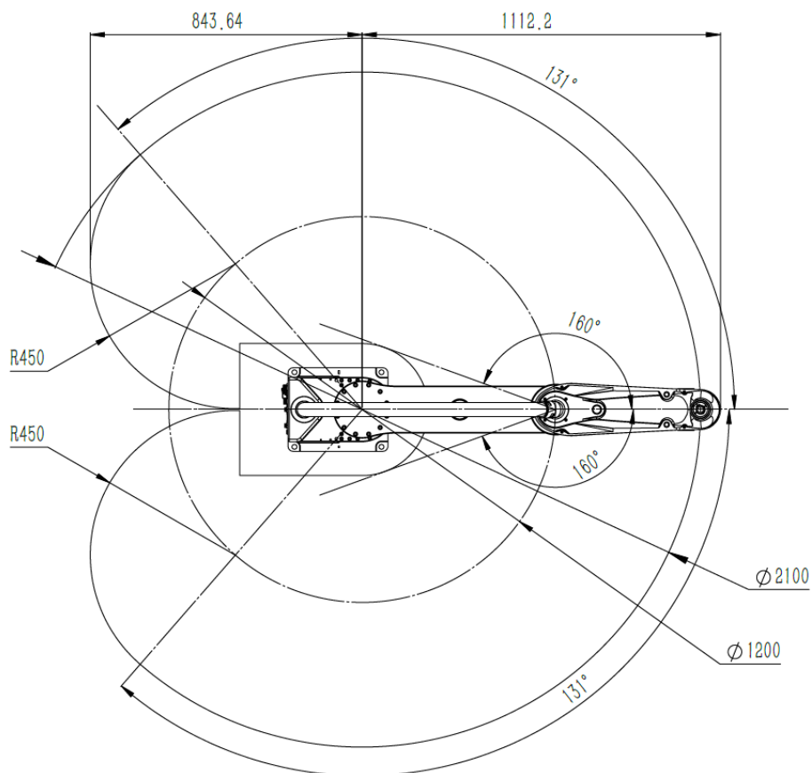
图 3-5 AH20-1050-0204-2000 / AH20-1050-0204-4000
